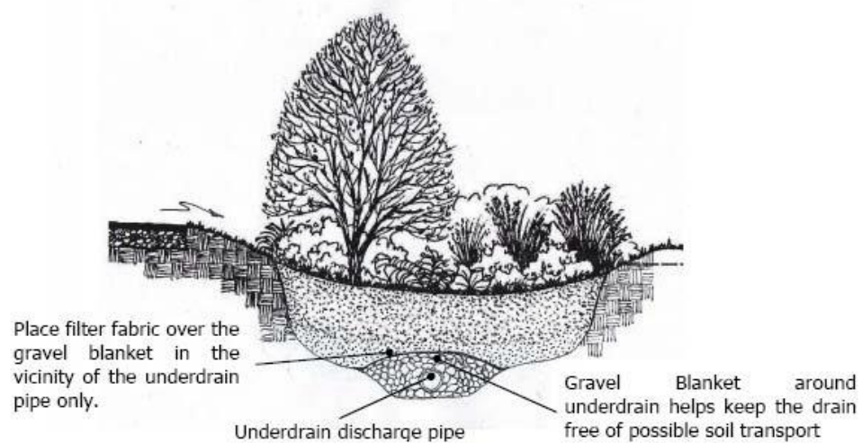
Figure PTP-10- 1 Filtration/Partial Recharge Facility
