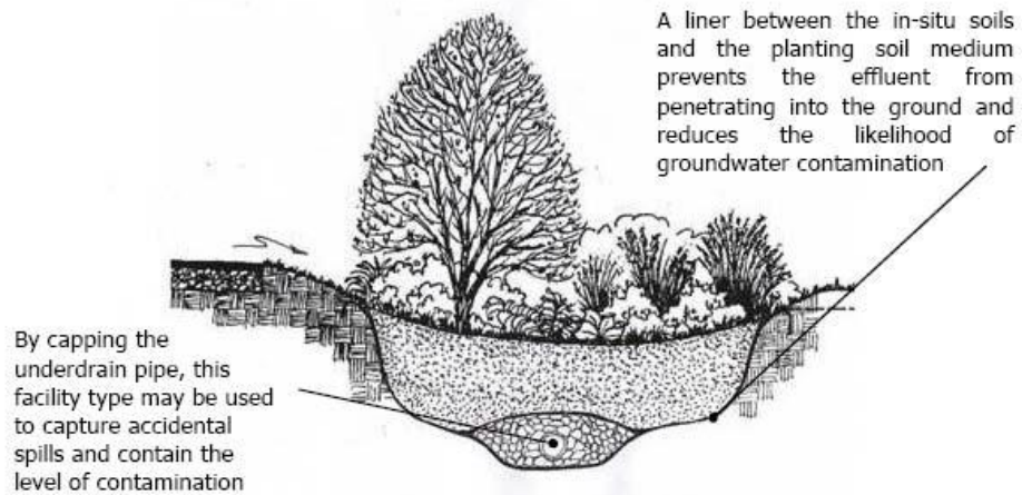
Figure PTP-10- 3 Filtration Only Facility
