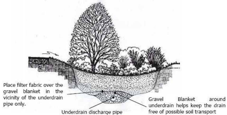
Figure PTP-10- 1 Filtration/Partial Recharge Facility Source, Minnesota Stormwater Manual
