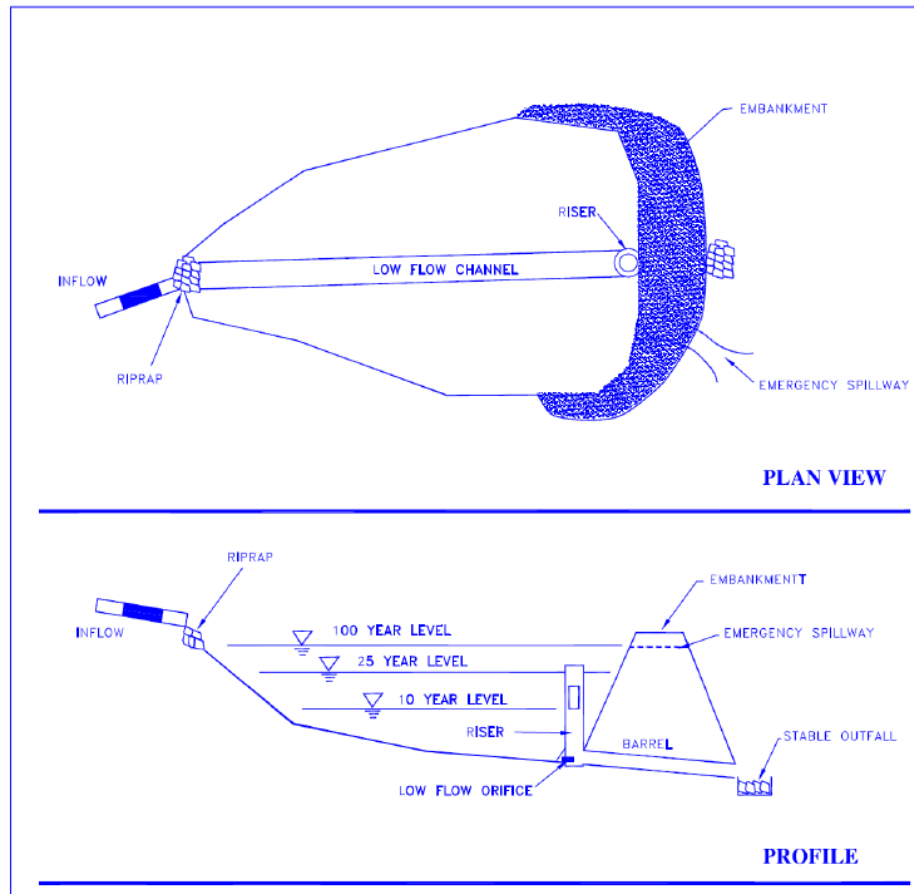
Figure PTP-08- 1 Detention Pond
