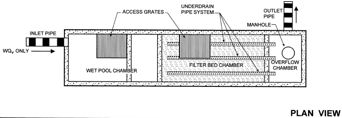
Figure PTP-01-13 Underground Sand Filter Source, Georgia Stormwater Management Manual
